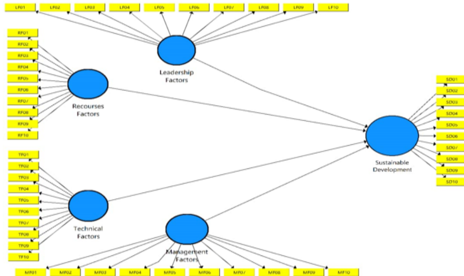
Figure 2: Hypothesized Model
